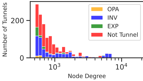
Figure 10: The degree distribution for HDNs with a degree over 512 either not in an MPLS tunnel, in an invisible (INV) tunnel, in an explicit tunnel (EXP), or in an opaque tunnel (OPA).
